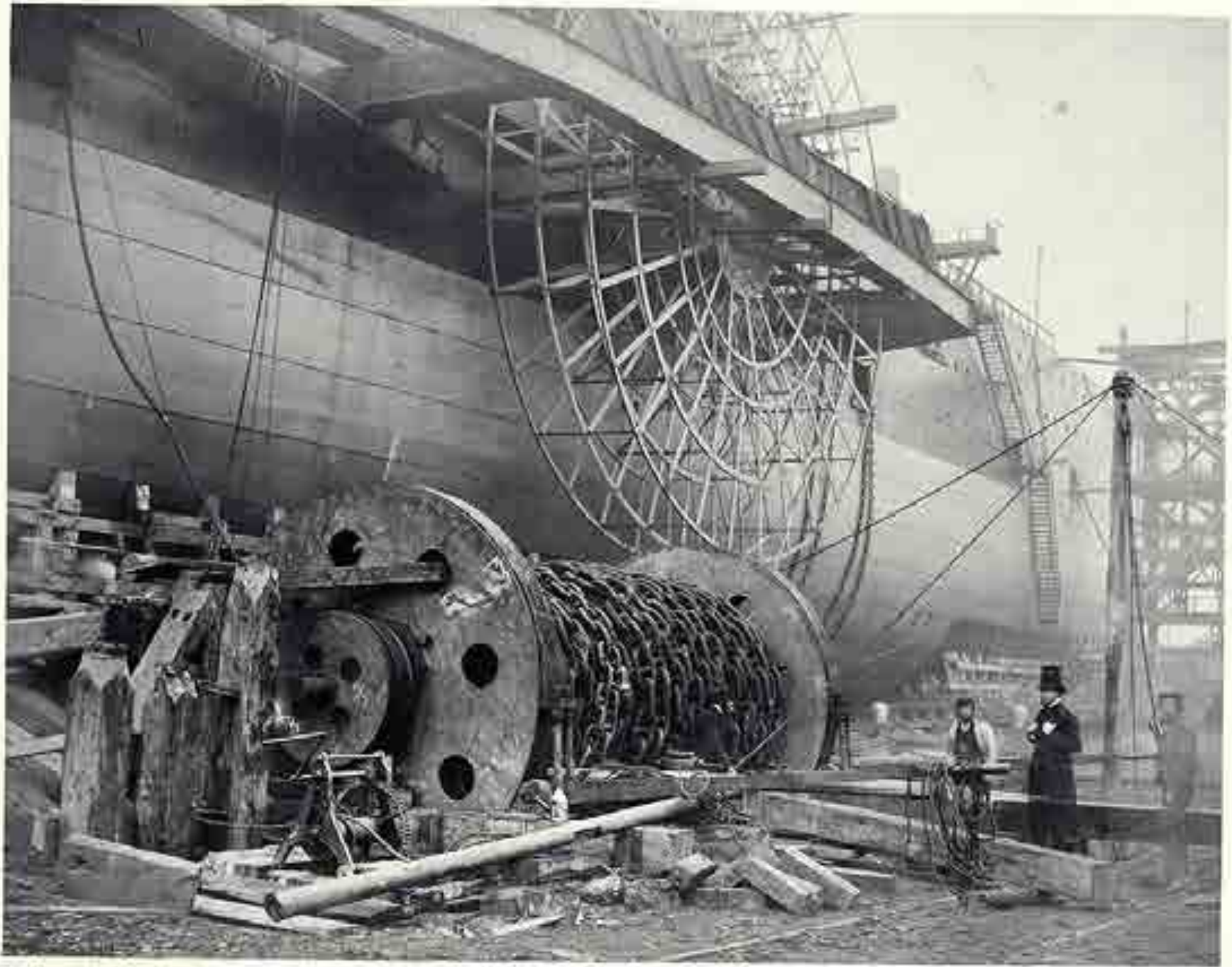
Robert Howlett, The Great Eastern Under Construction , 1857
